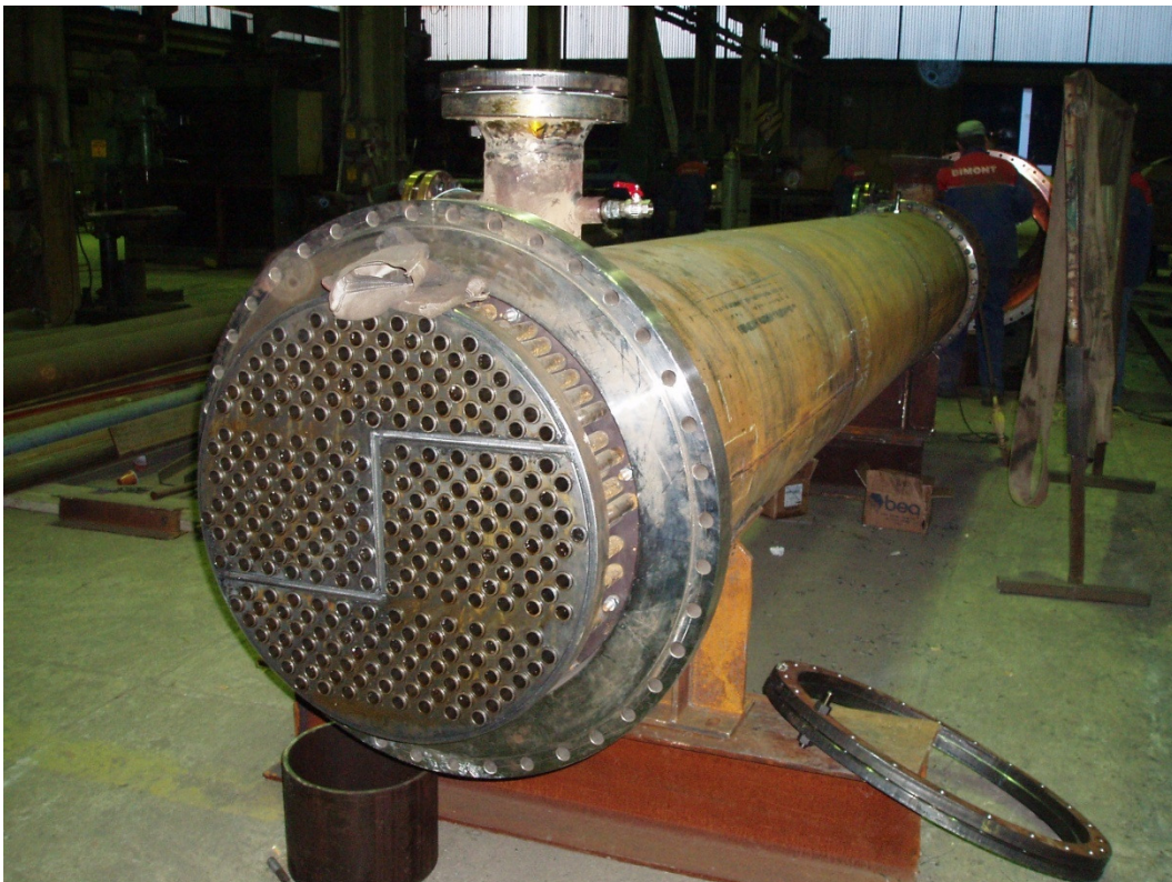
Heat Exchanger
